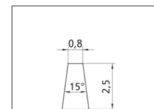
Depth: 100 mm Profile No. 2.3.2.008.020
