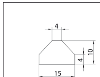
Depth: 25 mm Profile No. 2.3.3.004.005
