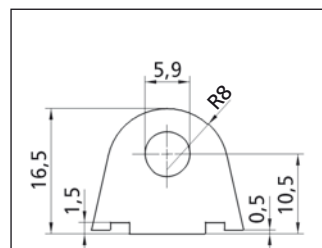
Depth: 15 mm Profile No. 2.3.3.016.032
