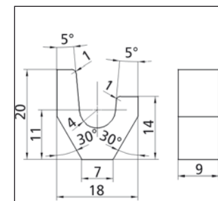
Profile No. 2.3.2.018.020
