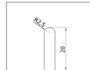
Depth: 100 mm Profile No. 2.3.2.008.010
