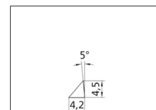
Profile No. 2.3.2.018.020
