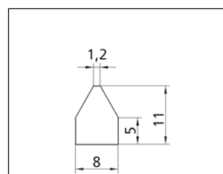
Depth: 100 mm Profile No. 2.3.3.023.036
