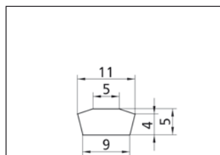
Depth: 15 mm Profile No. 2.3.3.013.024
